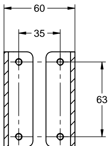
Fastening Plate
